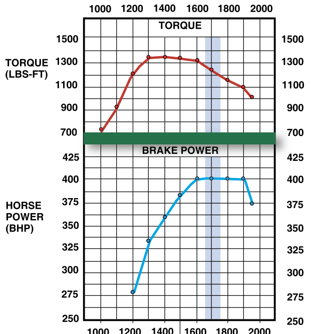
AI-375A POWER CURVE for Allison Transmission
