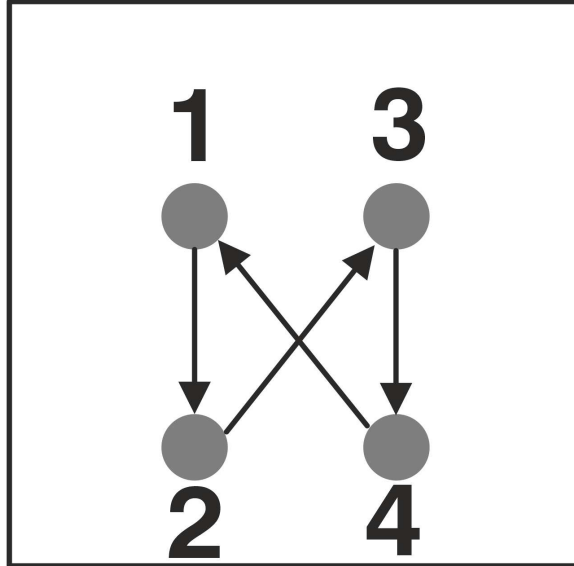
Torquing Sequence
